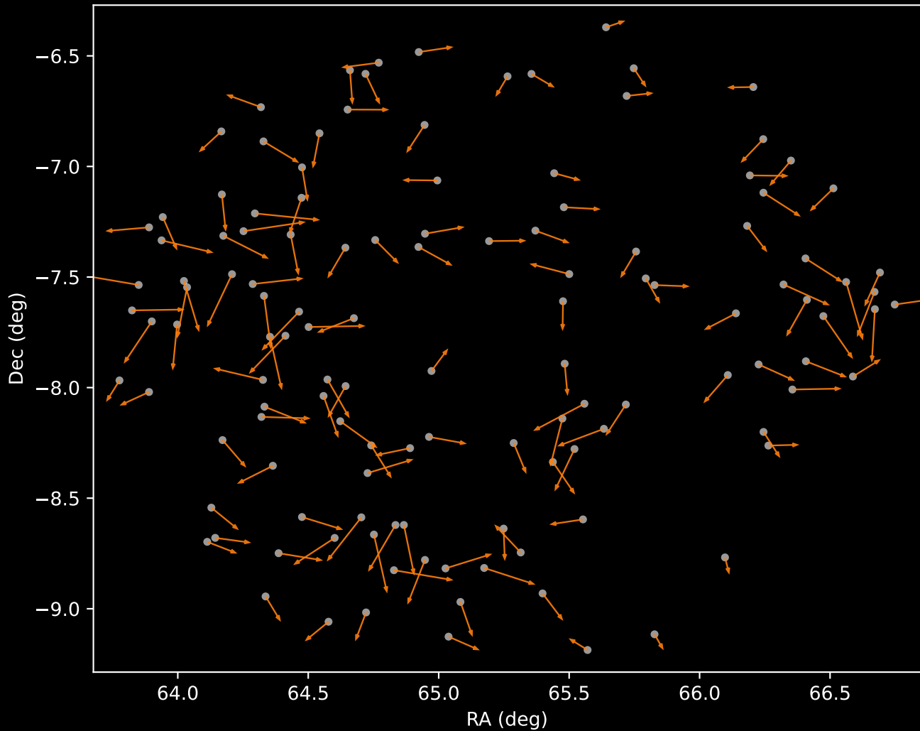
APOGEE DR17 Cluster 2 Proper Motion Vectors (n=127)
