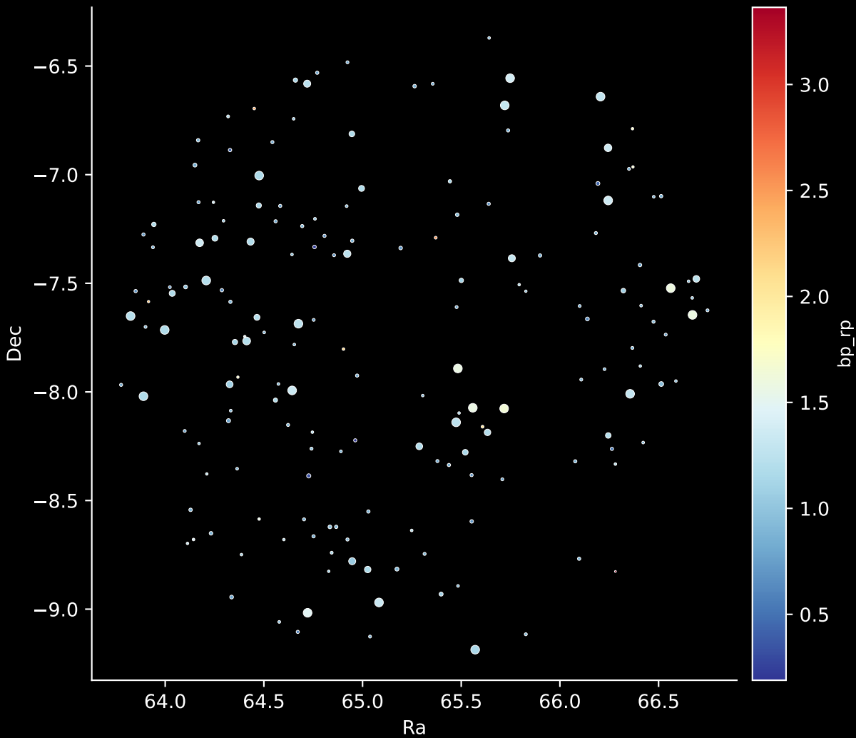
APOGEE DR17 Field: [047-41_MGA] Stars: 174
