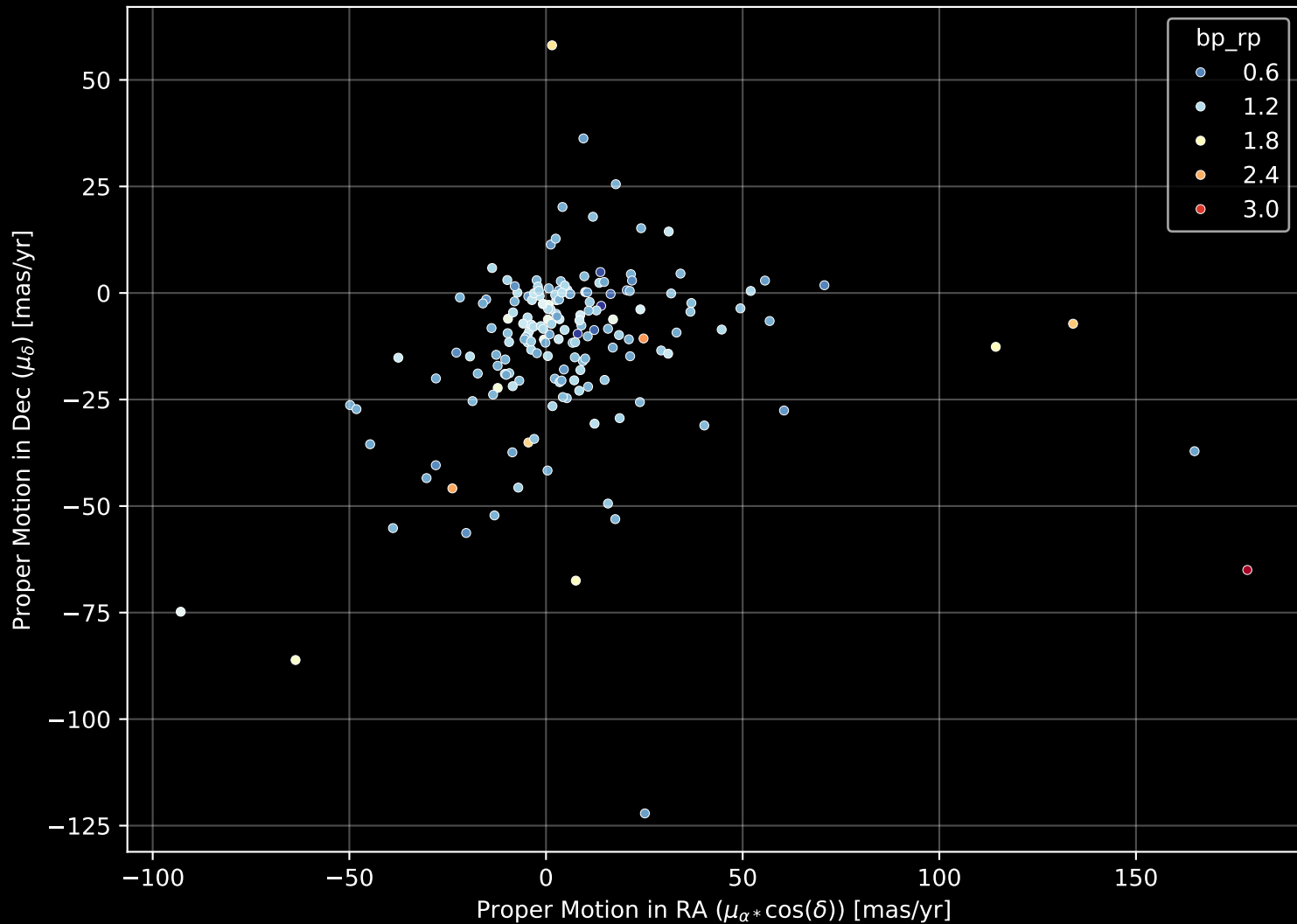
APOGEE DR17 Field: [047-41_MGA] Proper Motion Diagram (n= 174)
