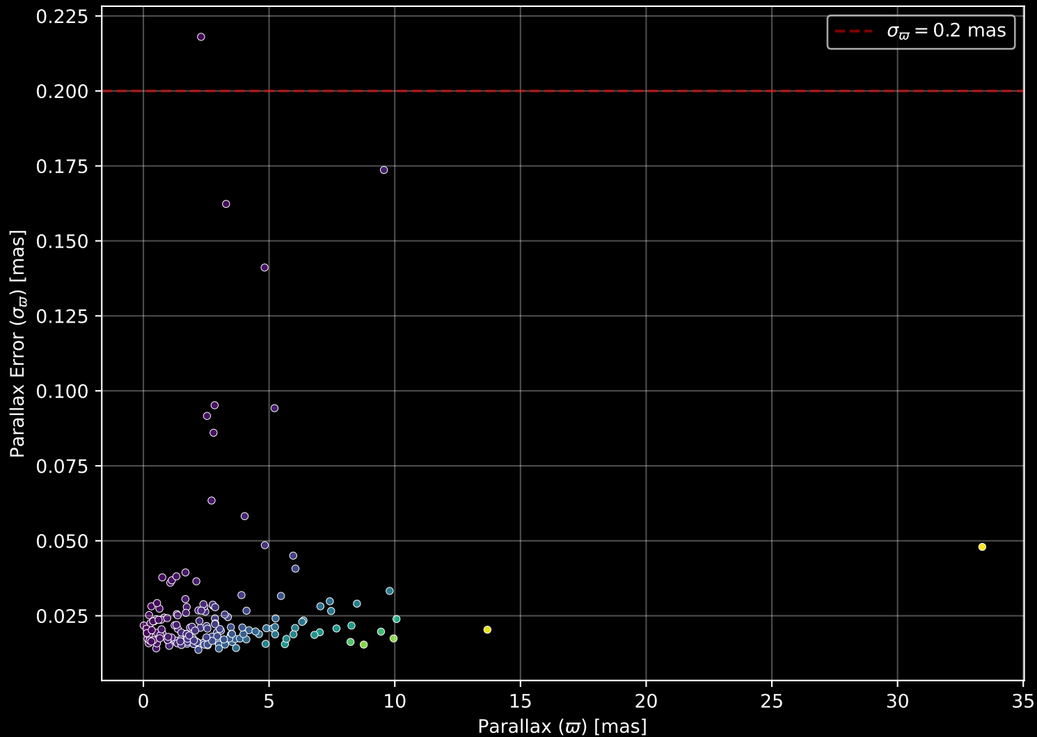
APOGEE DR17 Field: [047-41_MGA] Parallax Quality (n= 174)
