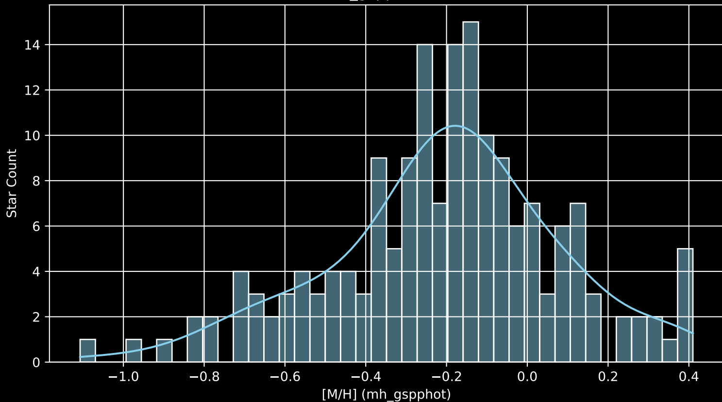
APOGEE DR17 Field: [047-41_MGA [M/H] (mh_gspphot) (n= 173)
