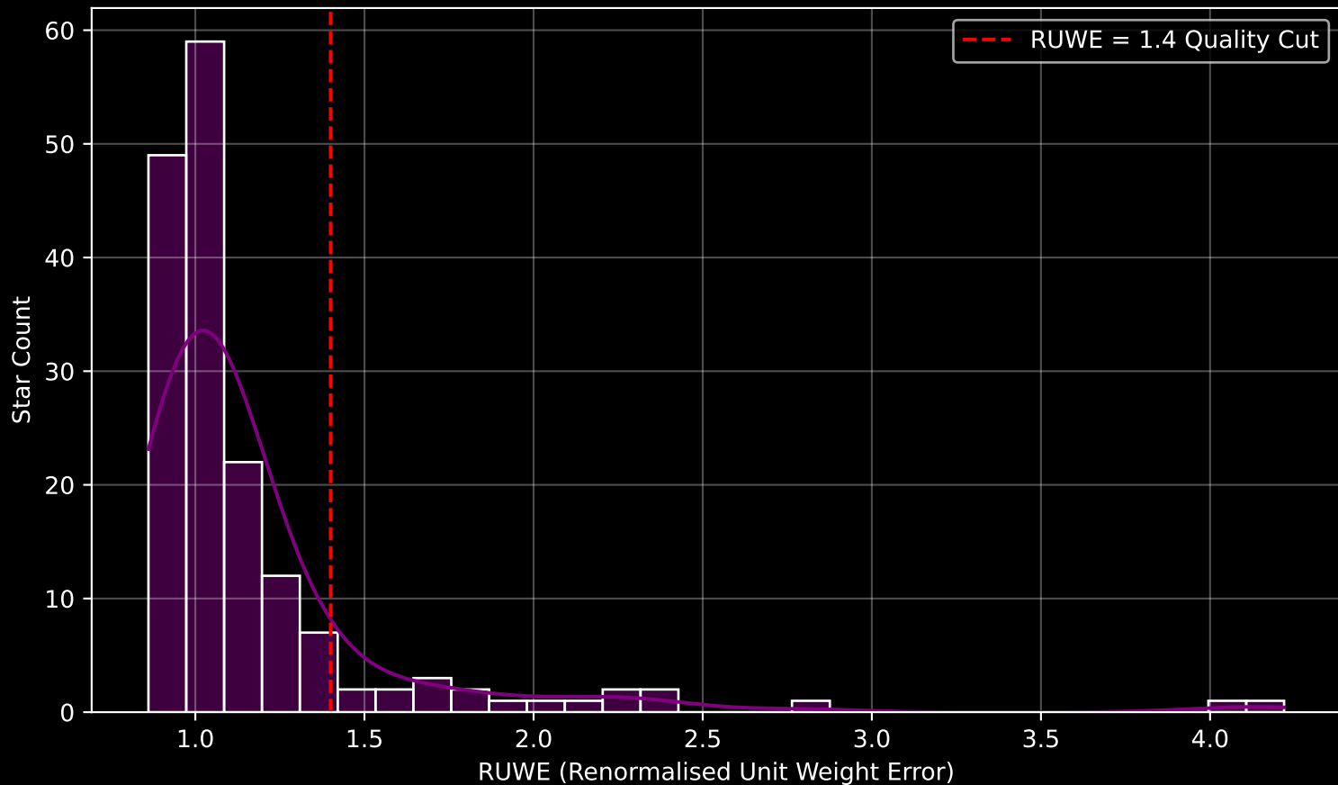
GAPOGEE DR17 Field [047-41_MGA] RUWE Distribution (n= 168)
