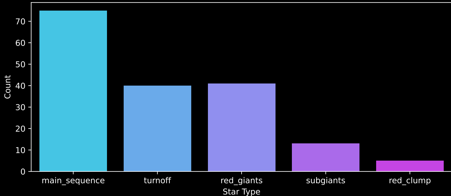
APOGEE DR17 Field: [047-41_MGA] Count plot of Star Type
